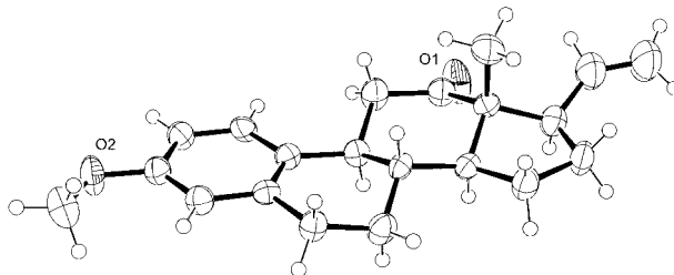
Figure 8. ORTEP diagram of steroid 11ad
