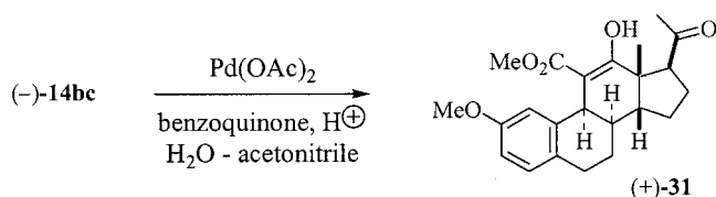
Scheme 15
