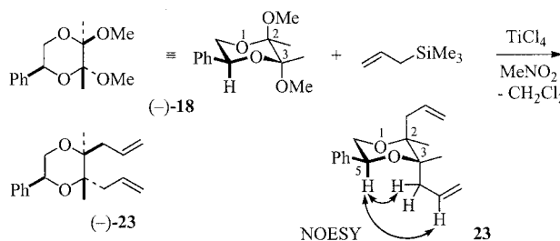
Scheme 8
