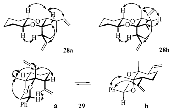
Figure 5. NOESY analyses of 28a , 28b , and 29
