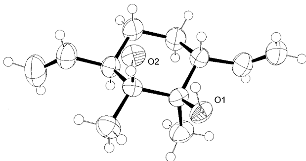
Figure 4. ORTEP diagram of diol ( \pm )- 27b
