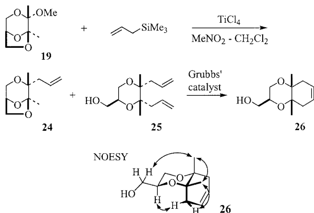
Scheme 9
