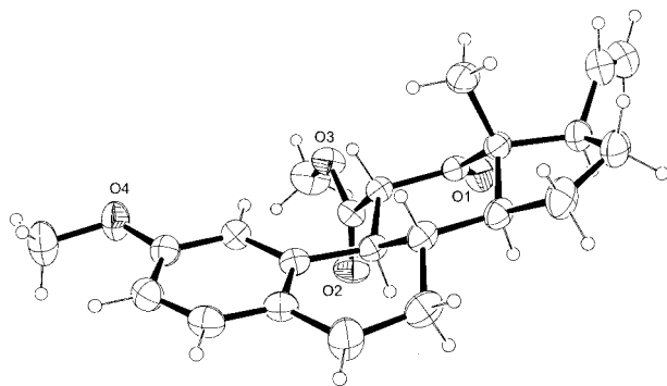
Figure 6. ORTEP diagram of steroid 10ac
