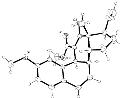
Figure 9. ORTEP diagram of steroid 14bc
