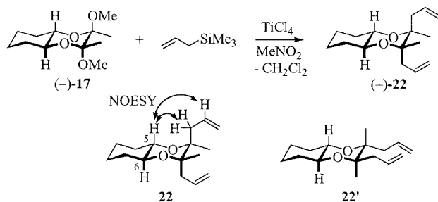
Scheme 6
