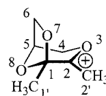
Figure 3. Optimized geometry of the oxocarbenium ion at the B3LYP/6.311G (d,p) level; selected bond lengths (Å): C(1)–O(8), 1.400; C(1)–O(7), 1.429; C(1)–C(2), 1.542; C(1)–C(1'), 1.505; C(2)–O(3), 1.270; C(2)–C(2'), 1.471; O(3)–C(4), 1.498; C(2)–O(7), 2.27; selected bond angles ( ^\circ ): O(7)–C(1)–C(2), 90.7; O(8)–C(1)–C(2), 108.6; O(7)–C(1)–O(8), 107.0; O(7)–C(1)–C(1'), 112.7; C(1)–C(2)–O(3), 119.3; C(1)–C(2)–C(2'), 123.8; C(2')–C(2)–O(3), 116.8; selected dihedral angles ( ^\circ ): O(8)–C(1)–C(2)–O(3), 30.3; C(1')–C(1)–C(2)–C(2'), -27.3; C(1)–C(2)–O(3)–C(4), -3.0; selected total atomic charges: C(1), -1.078; C(1'), -0.577; C(2), 0.770; C(2'), -0.686; O(3), 0.104; O(7), 0.063; O(8), 0.018; the HOMO (MO, 38; E = -12.36 eV) is centered on O(7) and the LUMO (MO, 39; E = -7.42 eV) is centered on C(2); total energy: -498.883(61) hartrees
