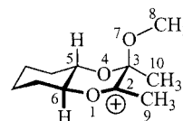
Figure 1. Optimized geometry of the oxocarbenium ion at the B3LYP/6.311G (d,p) level; selected bond lengths (Å): O(1)–C(2), 1.258; O(1)–C(6), 1.530; C(2)–C(3), 1.549; C(2)–C(9), 1.475; C(3)–O(4), 1.404; C(3)–O(7), 1.406; O(4)–C(5), 1.437; C(5)–C(6), 1.506; O(7)–C(8), 1.445; C(2)–O(7), 2.27; O(4)–O(7), 2.34; C(10)–O(7), 2.48; selected bond angles (°): O(1)–C(2)–C(3), 121.9; O(1)–C(2)–C(9), 116.9; C(3)–C(2)–C(9), 121.2; C(2)–C(3)–O(7), 100.4; O(4)–C(3)–O(7), 112.9; O(7)–C(3)–C(10), 115.2; selected dihedral angle (°): O(1)–C(2)–C(3)–O(4), –5.0; O(1)–C(2)–C(3)–O(7), 114.9; C(2)–C(3)–O(7)–C(8), 173.3; C(9)–C(2)–C(3)–O(7), –64.2; selected total atomic charges: O(1), 0.175; C(2), 0.398; C(9), –0.468; C(3), –0.709; O(4), 0.127; O(7), 0.001; C(8), –0.173; the HOMO (MO, 54; E = –11.76 eV) is centered on O(7) and the LUMO (MO, 55; E = –6.98 eV) is centered on C(2); total energy: –656.201(90) hartrees
